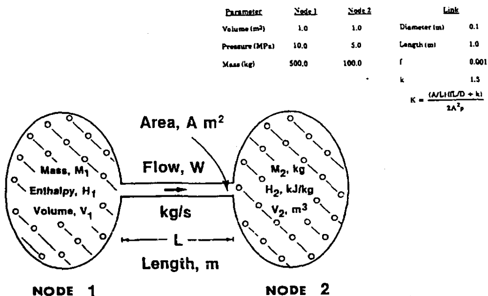
Figure 5.1 Simple 2-node, 1-link system.
